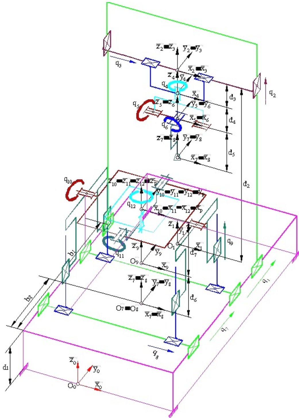
Fig. 2. The kinematical structure type 3T3R – 3T3R in the zero configuration
